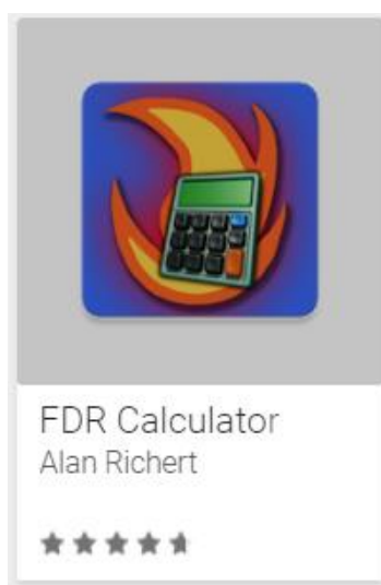
Figure 23- FDI calculator
