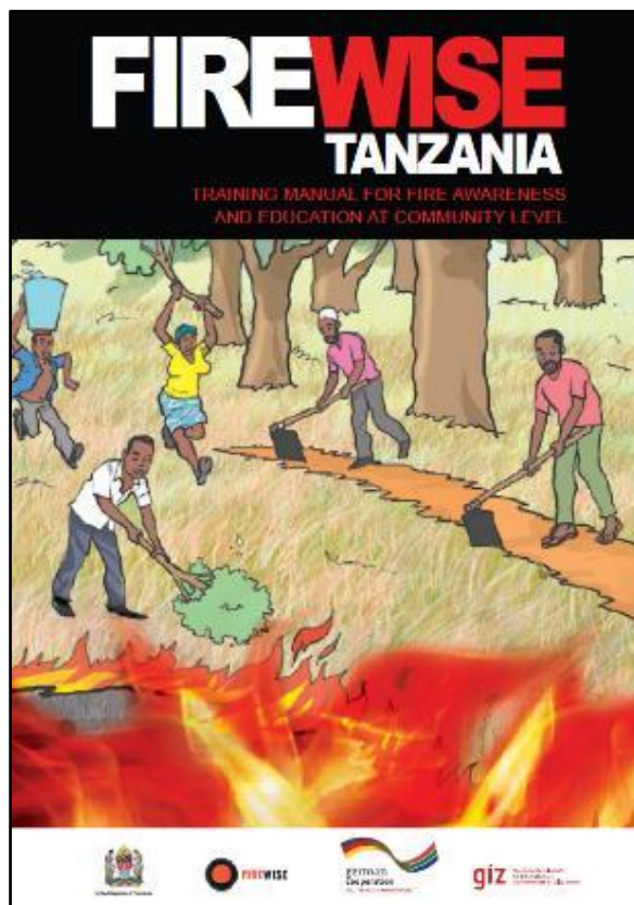
Figure 18- FireWise Tanzania
