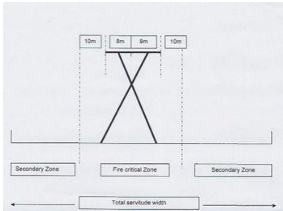
Figure 28- Typical cross section of powerline
